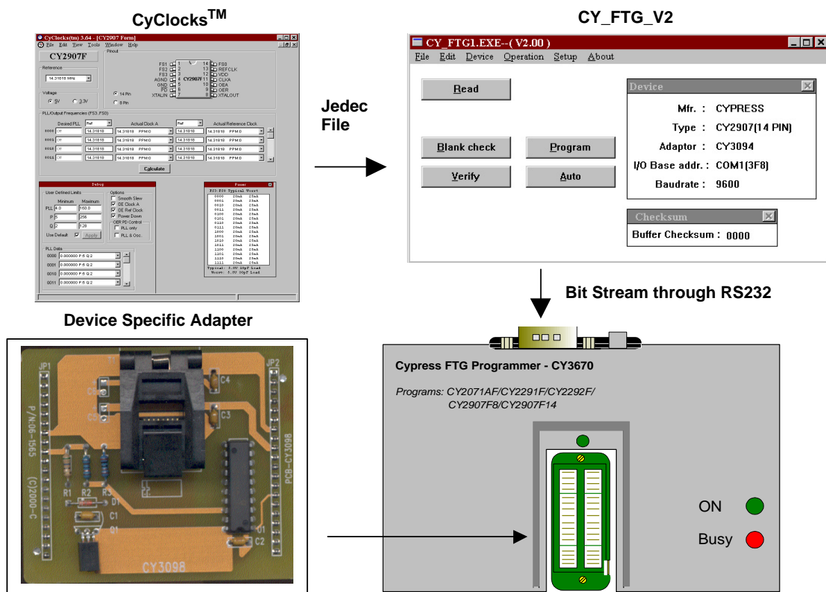
Figure 1. Programming Procedure
